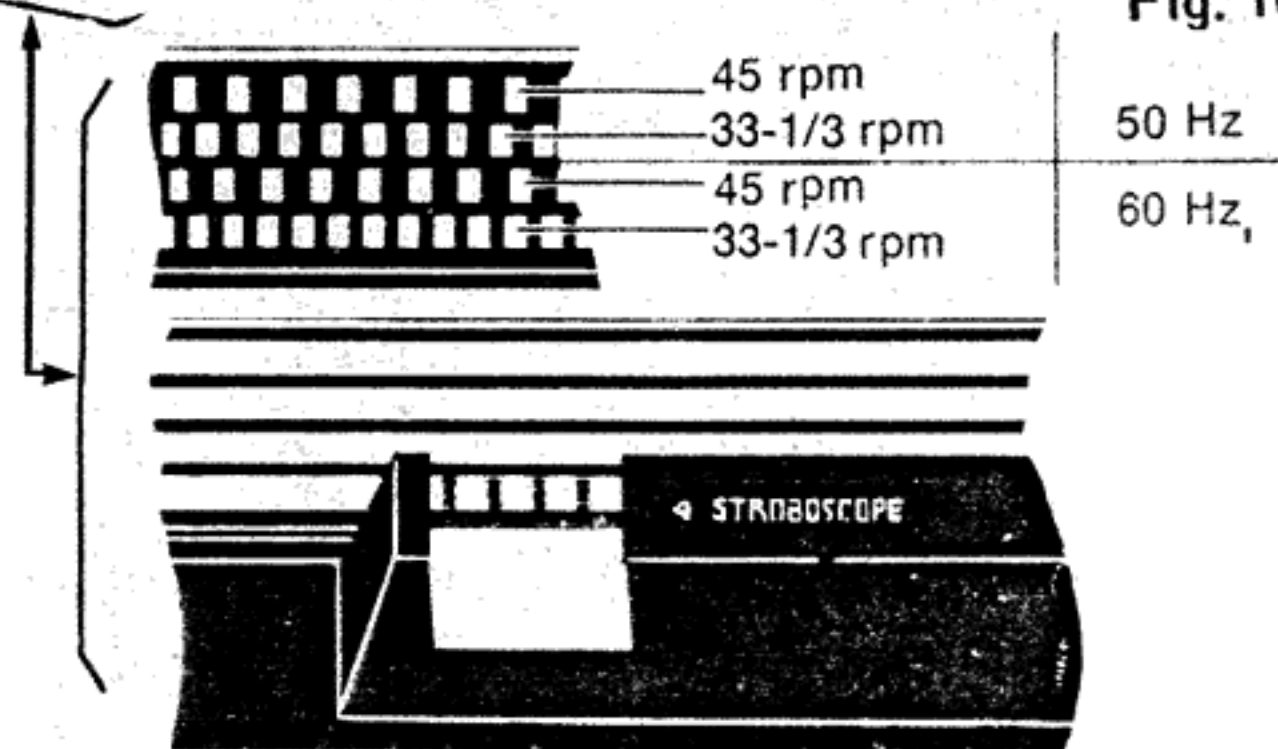
Strobe of 60 Hz, 33-1/3 rpm The strobe dots seem to be stationary.
