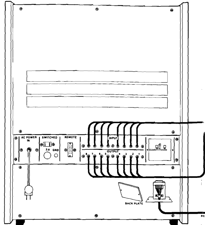
Fig. 31 DX-8 Connection
