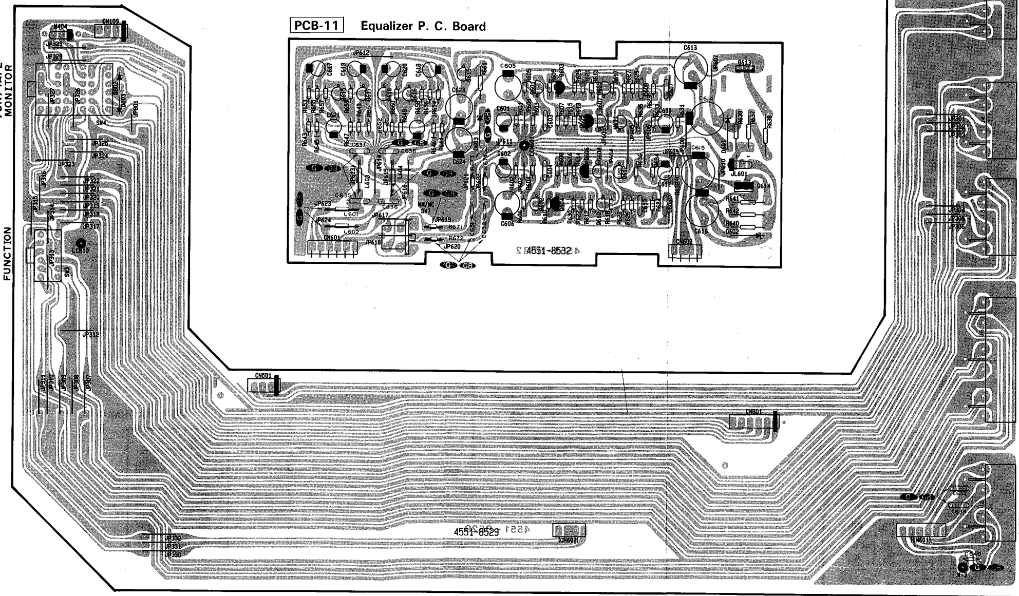
PCB-8 Function P. C. Board
